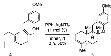
Scheme 3. Au-Catalyzed Cycloisomerization of 1,5,9-Dienyne 4
